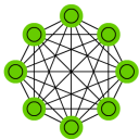
Markov Chain (MC)
