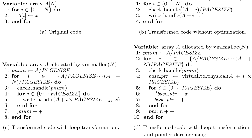
Fig. 5. Example of optimizations on an array accesses.
