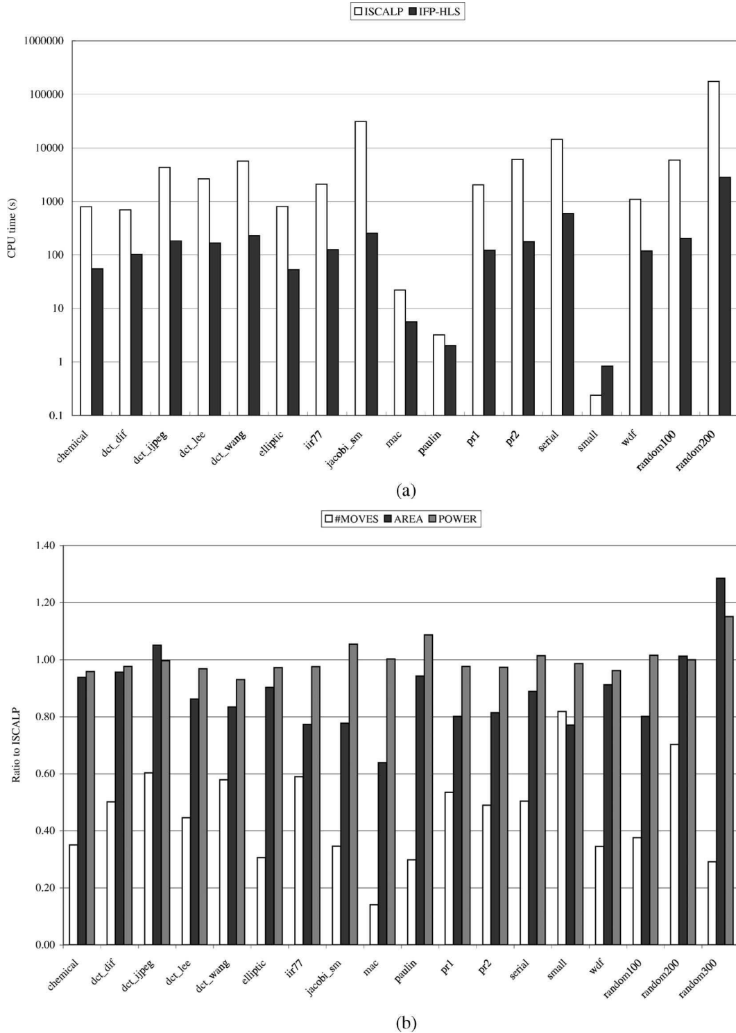
Fig. 8. Comparison between ISCALP and IFP-HLS for unity-aspect-ratio FUs. (a) CPU time for unity-aspect-ratio FUs. (b) Number of moves, area, and power consumption for unity-aspect-ratio FUs.
