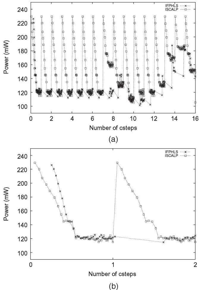
Fig. 1. Power consumption of intermediate solution during the optimization of ISCALP and IFP-HLS. (a) Power consumption of intermediate solution during the optimization for all the values of csteps . (b) Power consumption of intermediate solution during the optimization for the values of csteps from zero to two.
